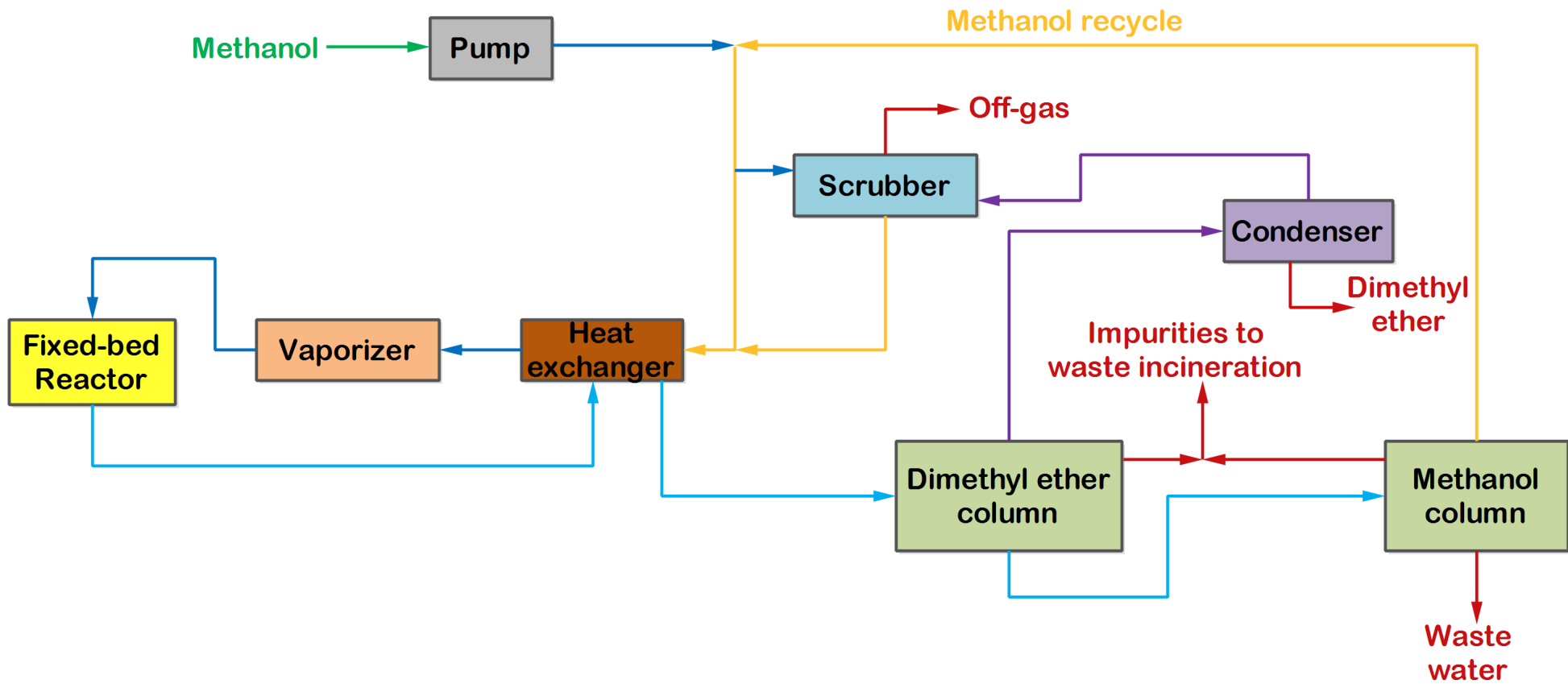
Figure: Manufacture of Dimethyl ether by dehydration of methanol
